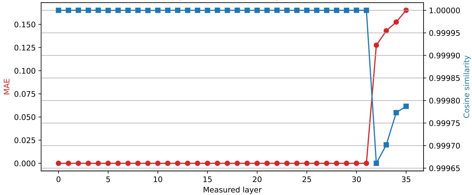
Qwen2.5-3B | Quantized layer 31 | float32 \rightarrow int8
