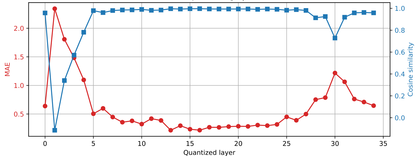
Qwen2.5-3B | Prompt 0 Final RMSNorm output damage | float32 \rightarrow int4
