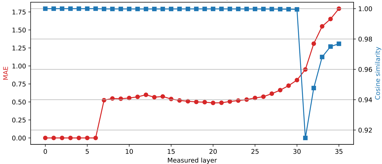
Qwen2.5-3B | Quantized layer 6 | float32 \rightarrow int4
