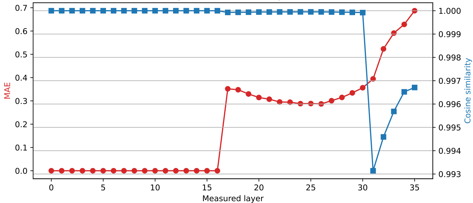
Qwen2.5-3B | Quantized layer 16 | float32 \rightarrow int4
