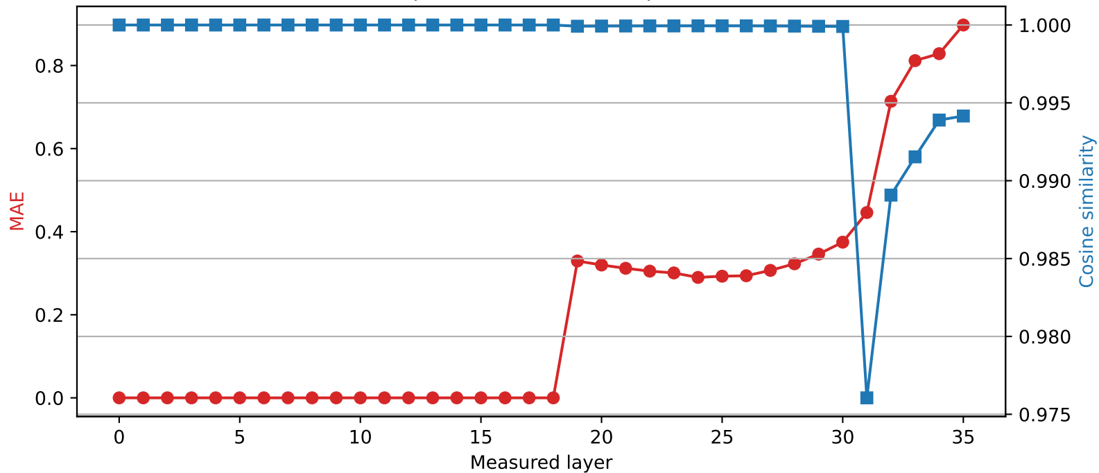
Qwen2.5-3B | Quantized layer 18 | float32 \rightarrow int4
