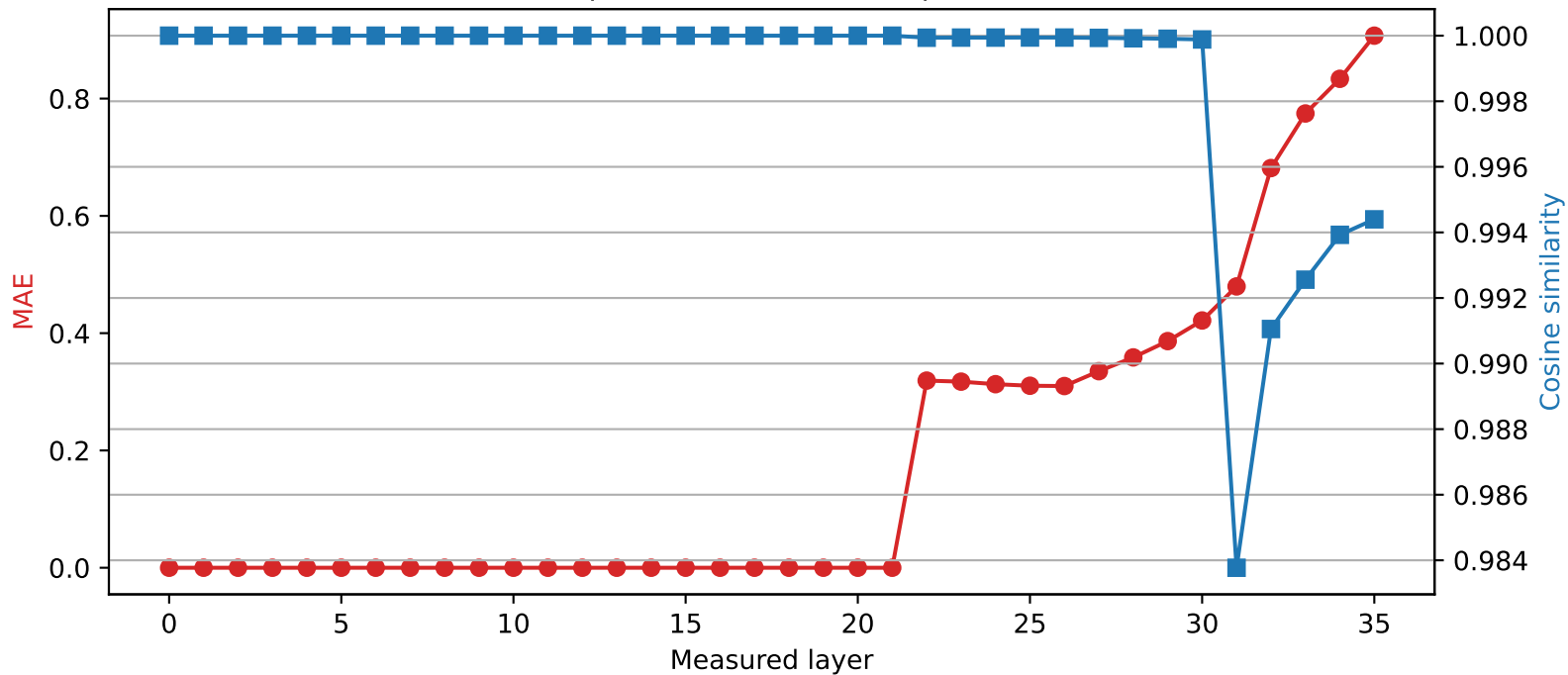
Qwen2.5-3B | Quantized layer 21 | float32 \rightarrow int4
