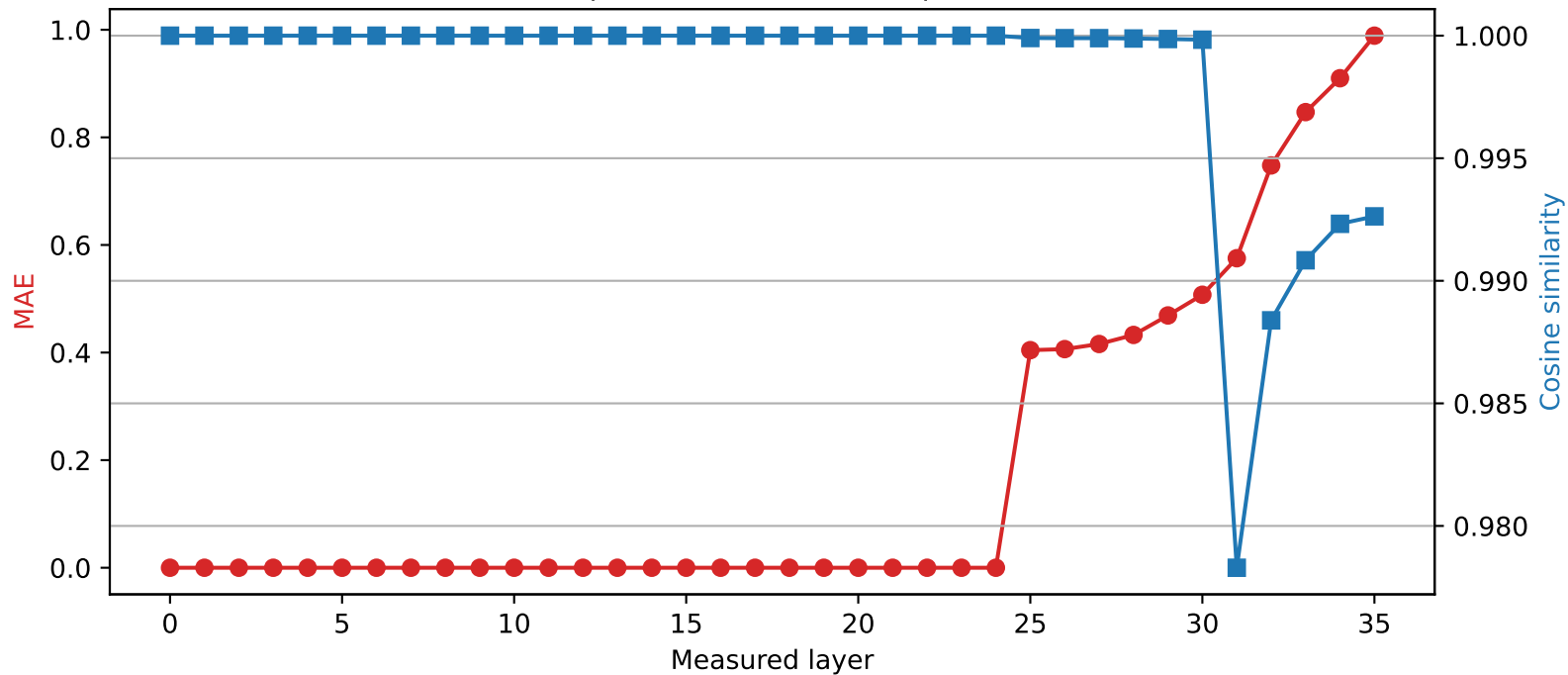
Qwen2.5-3B | Quantized layer 24 | float32 \rightarrow int4
