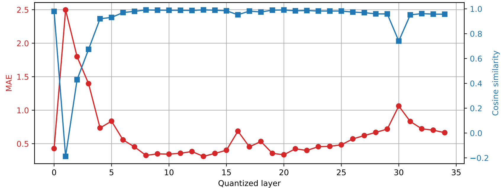
Qwen2.5-3B | Prompt 1 Final RMSNorm output damage | float32 → int4
