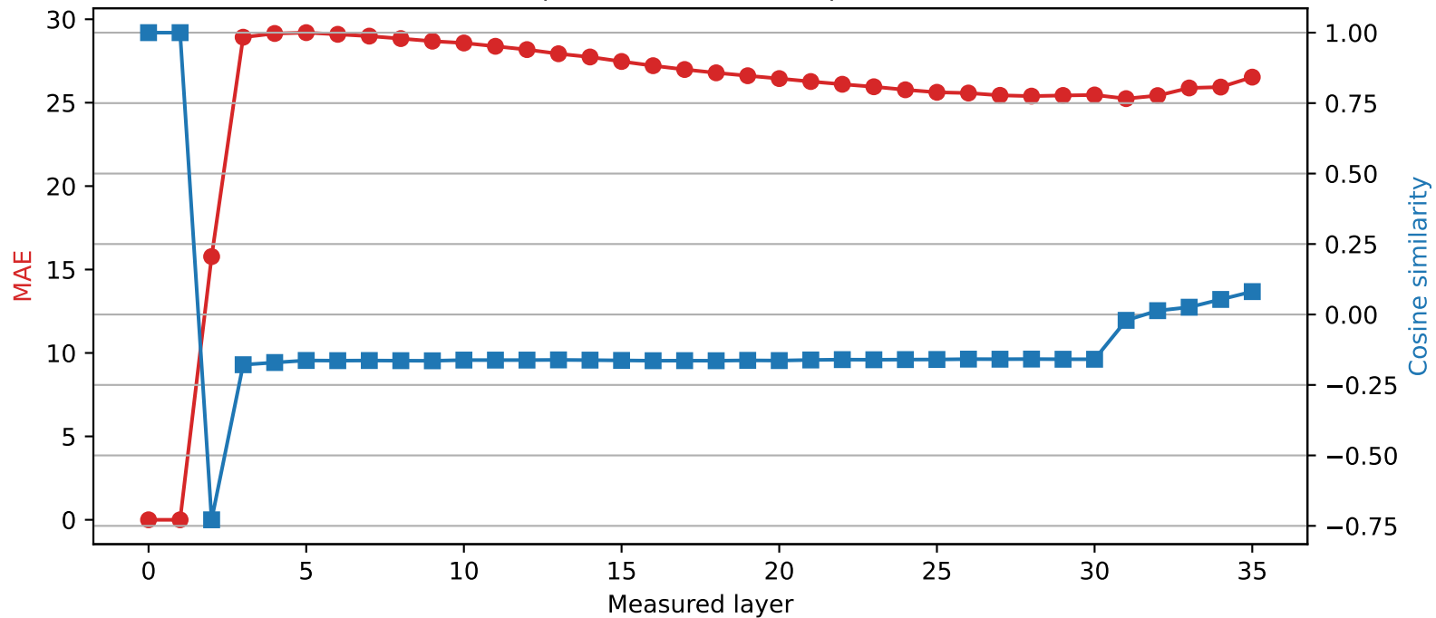
Qwen2.5-3B | Quantized layer 1 | float32 \rightarrow int4
