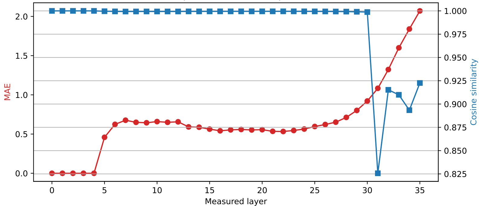
Qwen2.5-3B | Quantized layer 4 | float32 → int4
