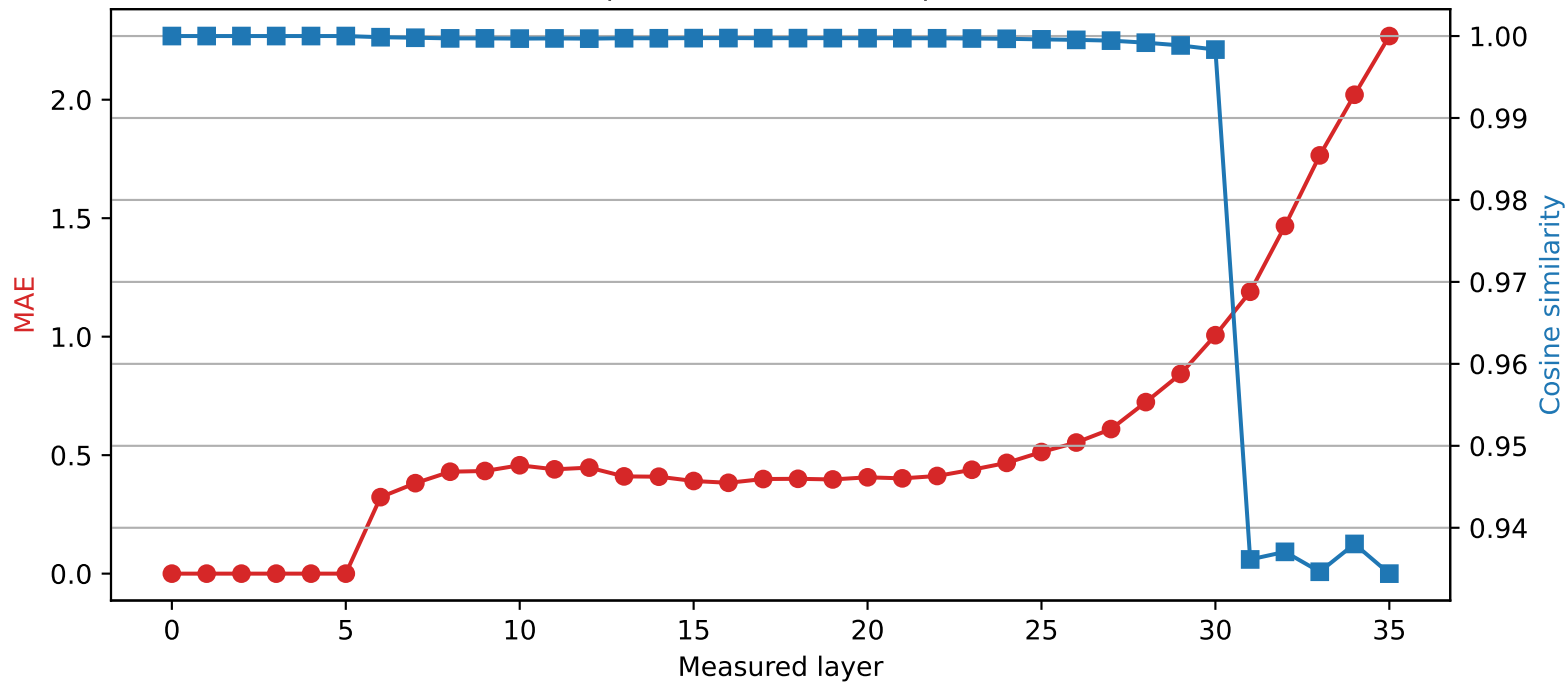
Qwen2.5-3B | Quantized layer 5 | float32 \rightarrow int4
