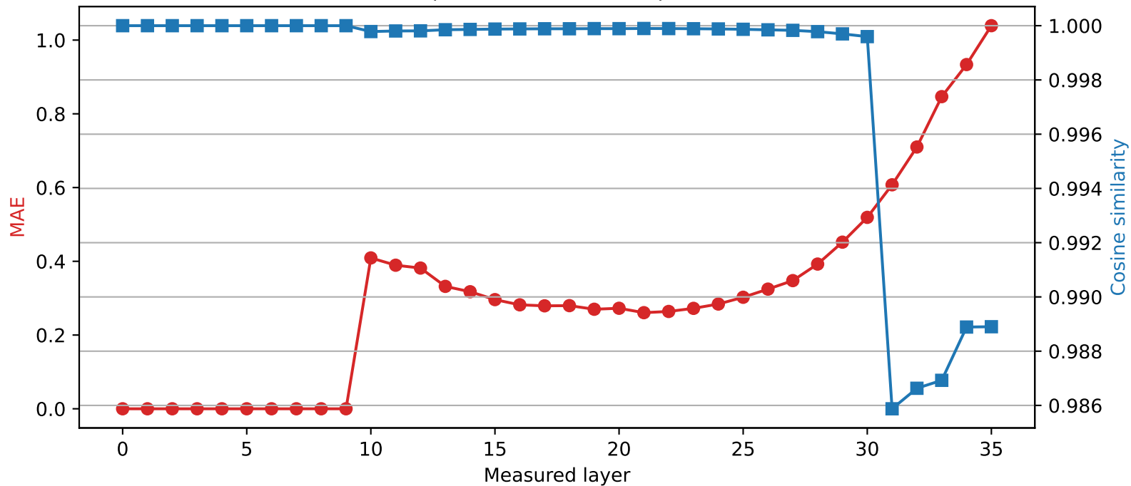
Qwen2.5-3B | Quantized layer 9 | float32 \rightarrow int4
