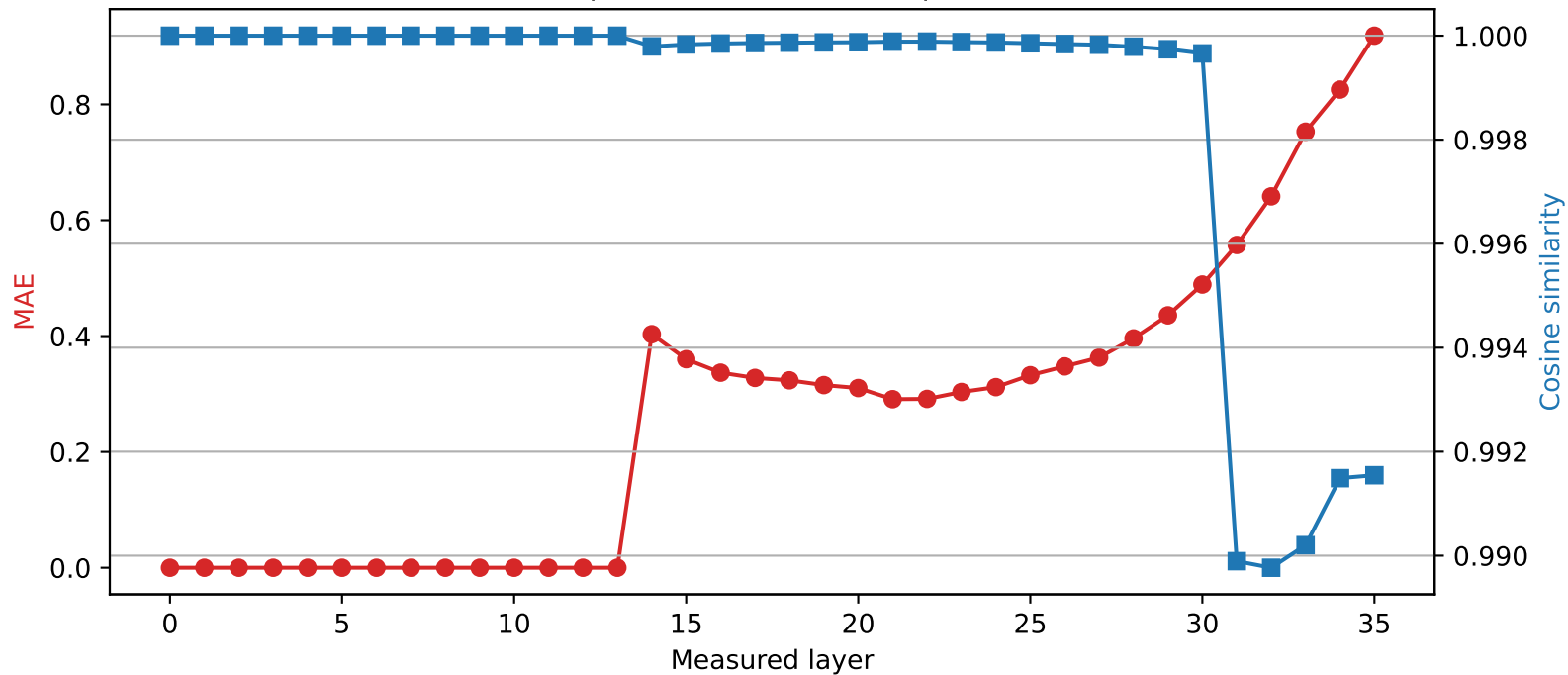
Qwen2.5-3B | Quantized layer 13 | float32 \rightarrow int4
