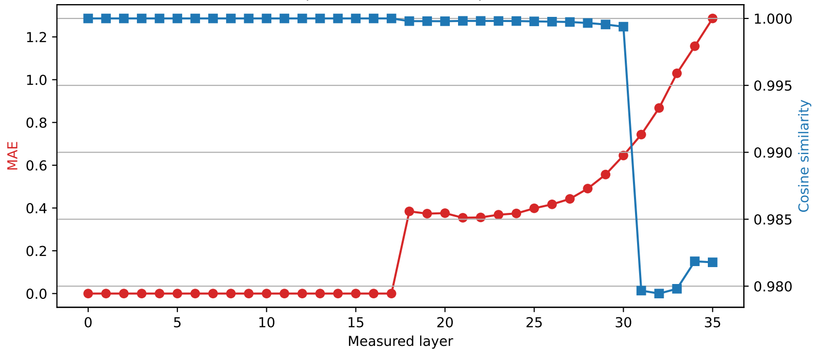
Qwen2.5-3B | Quantized layer 17 | float32 \rightarrow int4
