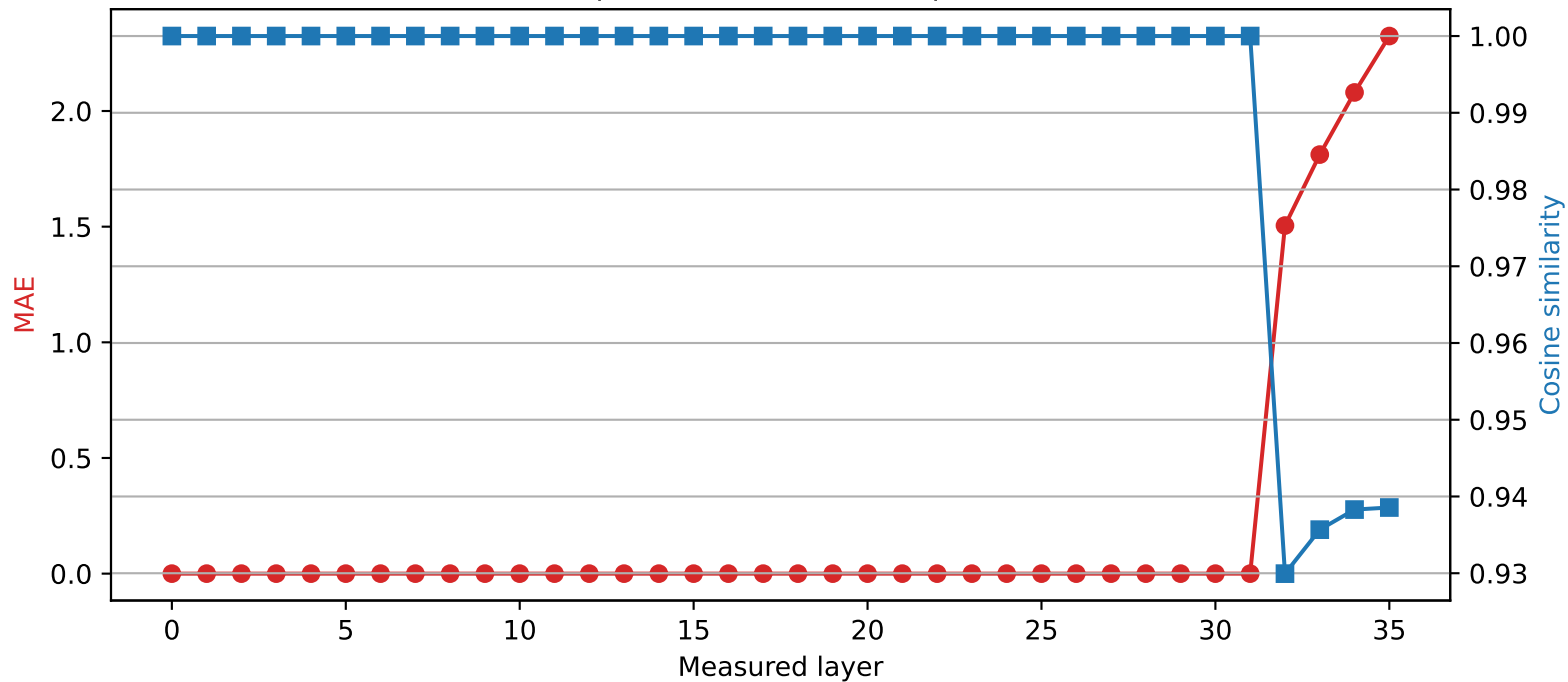
Qwen2.5-3B | Quantized layer 31 | float32 \rightarrow int4
