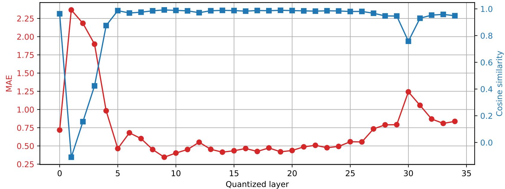
Qwen2.5-3B | Prompt 2 Final RMSNorm output damage | float32 \rightarrow int4
