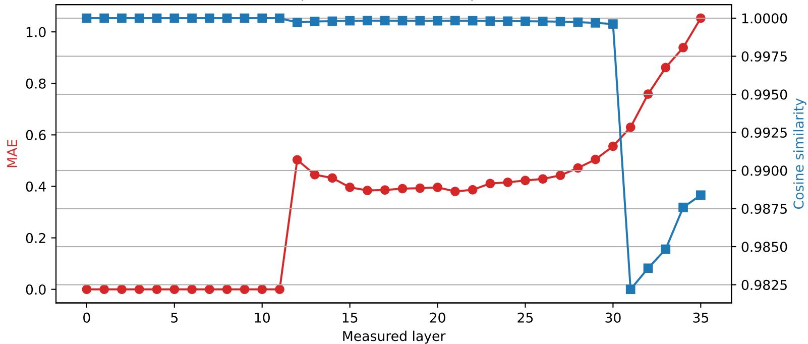
Qwen2.5-3B | Quantized layer 11 | float32 \rightarrow int4
