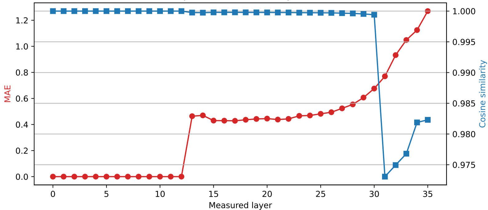
Qwen2.5-3B | Quantized layer 12 | float32 \rightarrow int4
