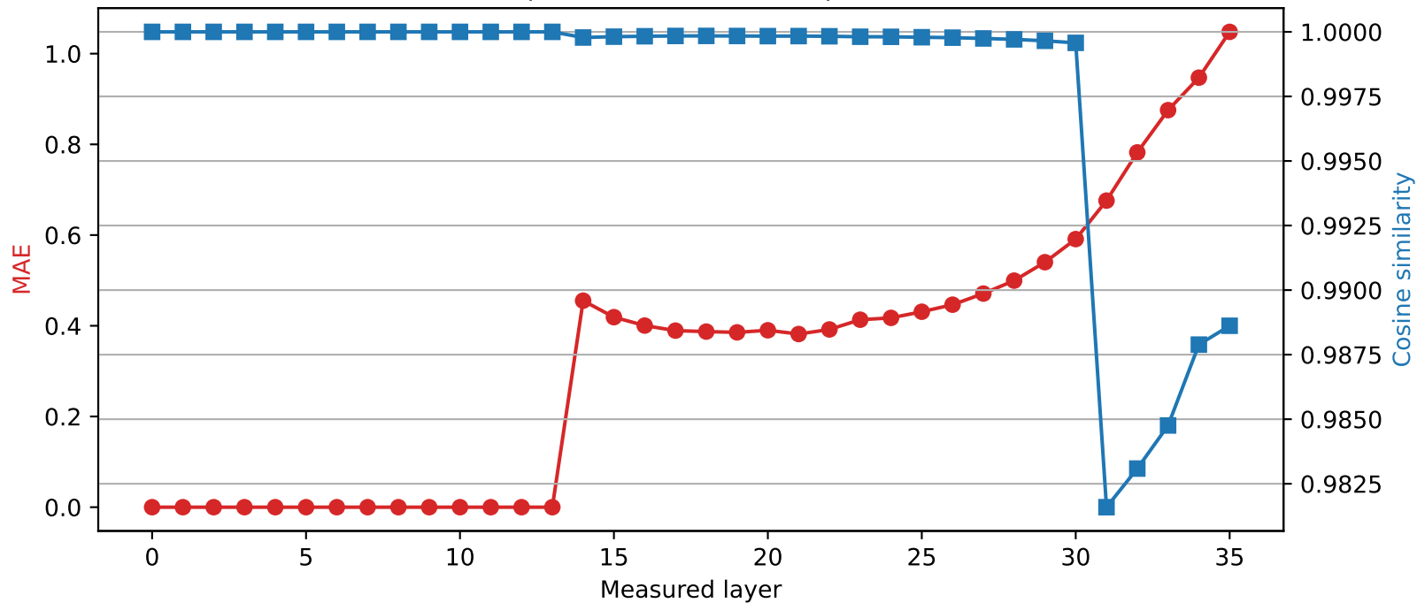
Qwen2.5-3B | Quantized layer 13 | float32 → int4
