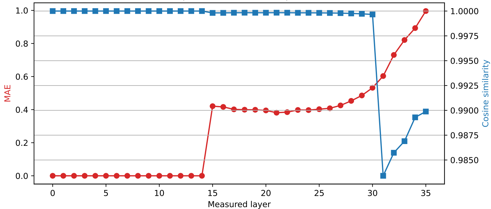
Qwen2.5-3B | Quantized layer 14 | float32 \rightarrow int4
