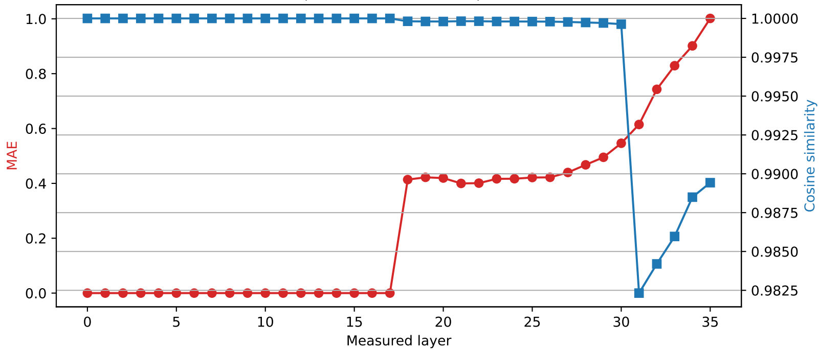
Qwen2.5-3B | Quantized layer 17 | float32 → int4
