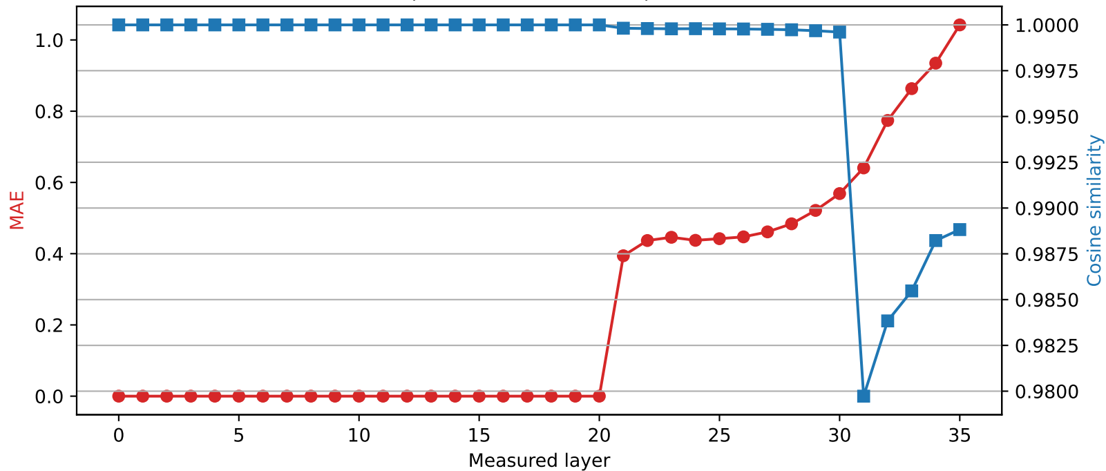
Qwen2.5-3B | Quantized layer 20 | float32 \rightarrow int4
