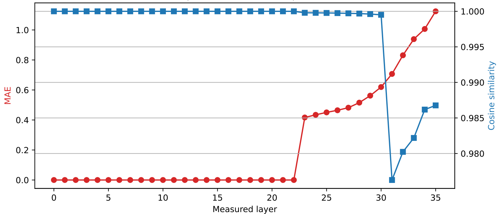
Qwen2.5-3B | Quantized layer 22 | float32 \rightarrow int4
