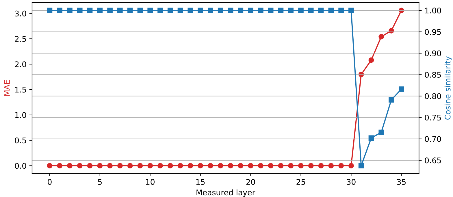
Qwen2.5-3B | Quantized layer 30 | float32 \rightarrow int4
