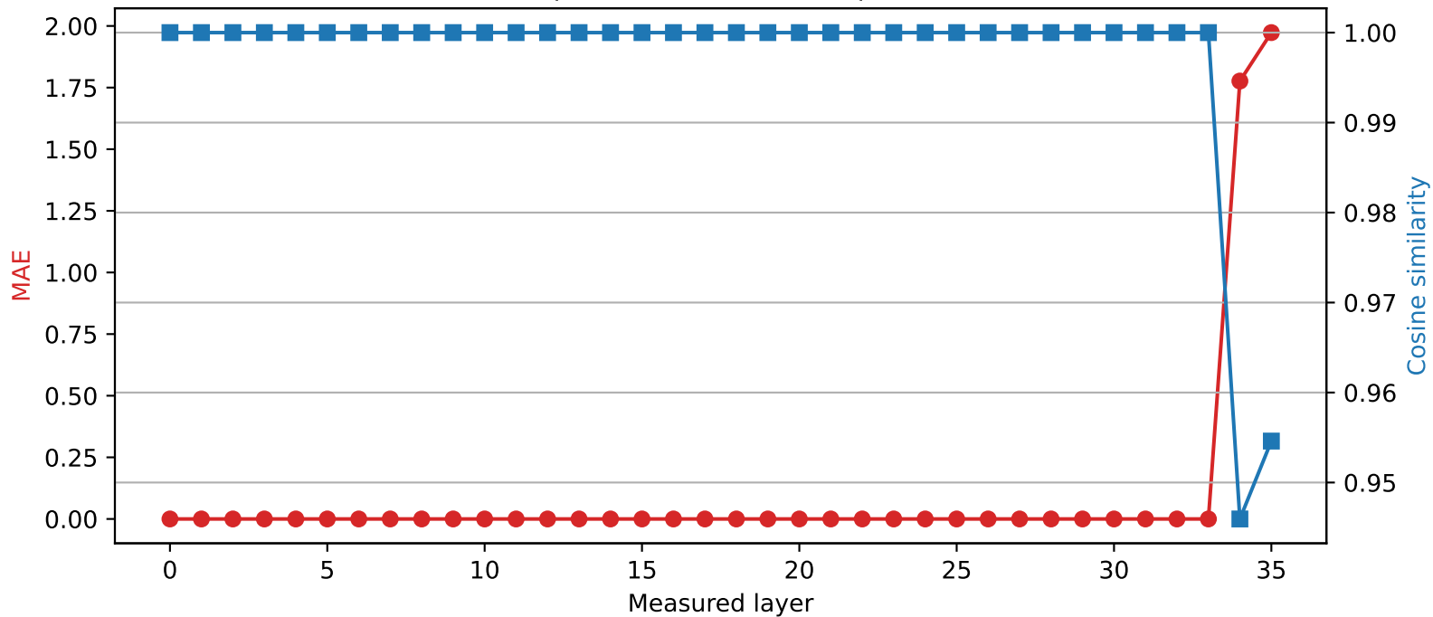
Qwen2.5-3B | Quantized layer 33 | float32 \rightarrow int4
