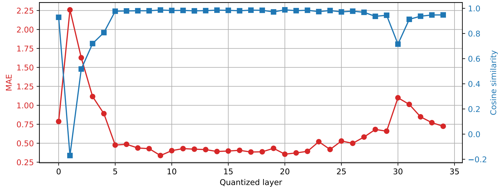
Qwen2.5-3B | Prompt 3 Final RMSNorm output damage | float32 \rightarrow int4
