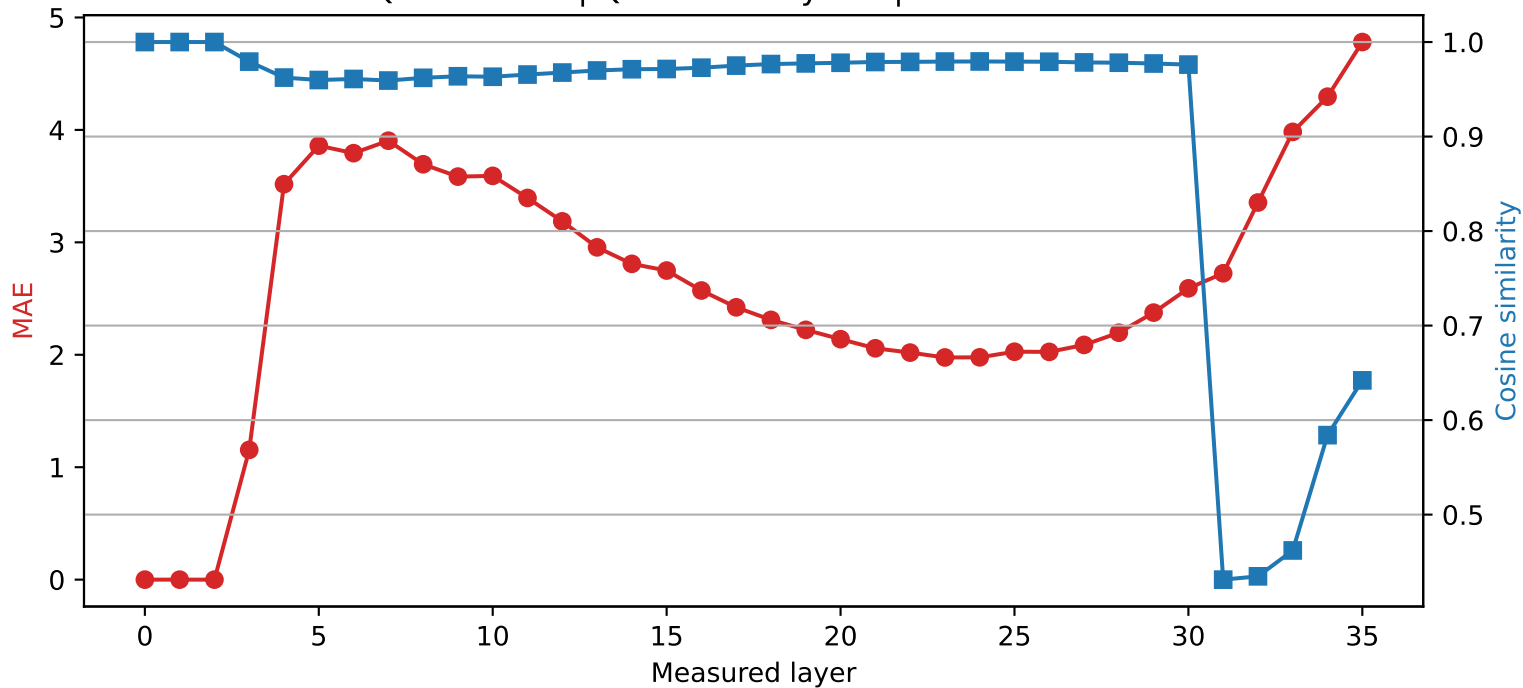
Qwen2.5-3B | Quantized layer 2 | float32 \rightarrow int4
