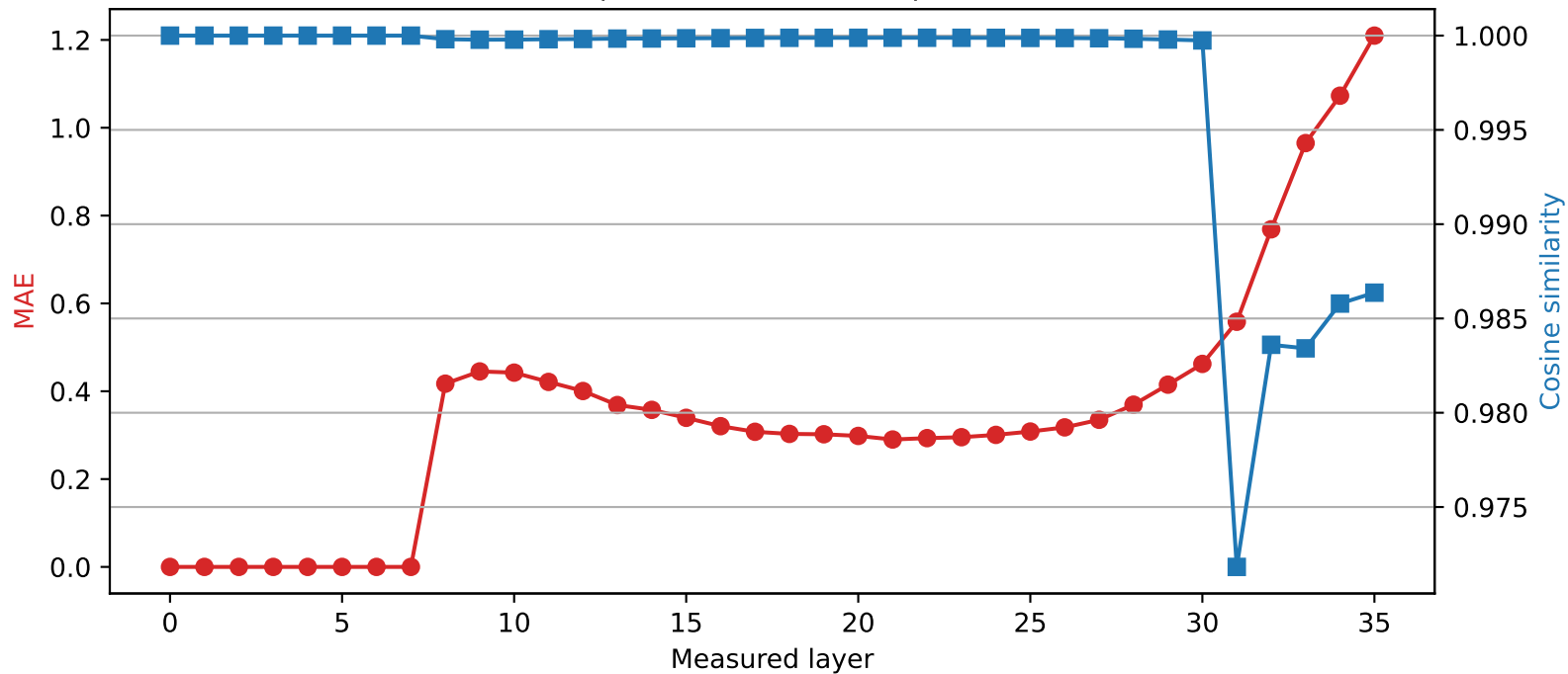
Qwen2.5-3B | Quantized layer 7 | float32 \rightarrow int4
