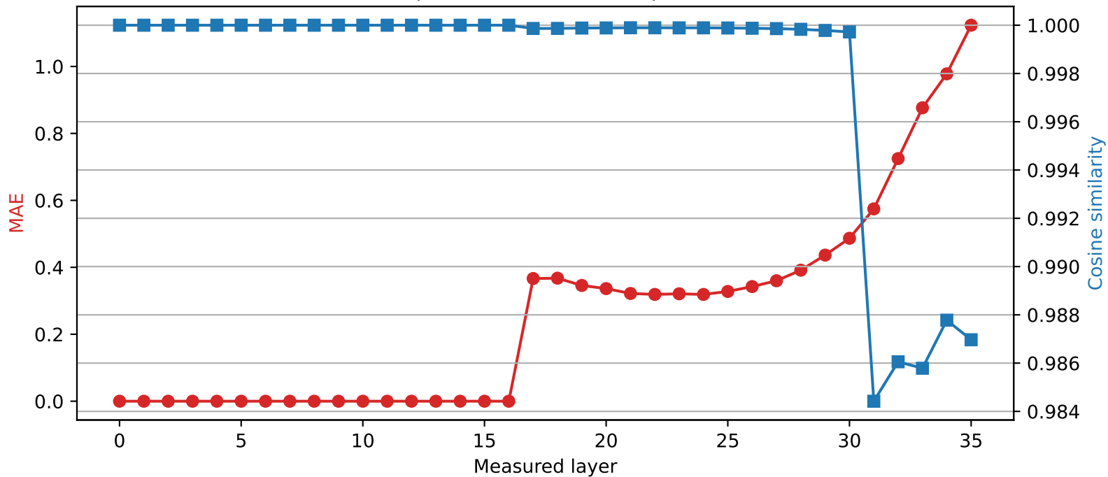
Qwen2.5-3B | Quantized layer 16 | float32 → int4
