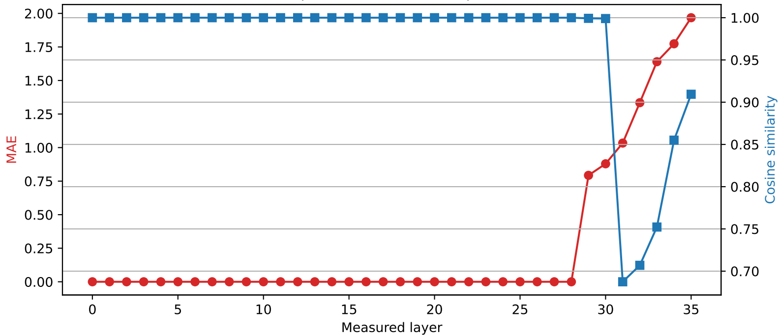
Qwen2.5-3B | Quantized layer 28 | float32 \rightarrow int4
