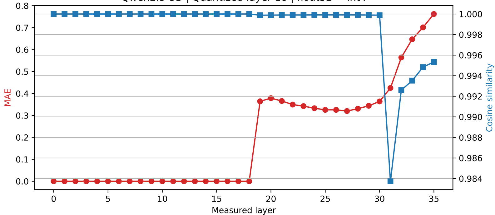
Qwen2.5-3B | Quantized layer 18 | float32 → int4
