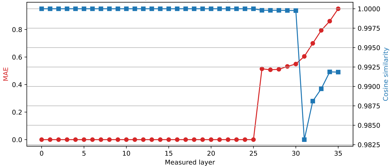
Qwen2.5-3B | Quantized layer 25 | float32 \rightarrow int4
