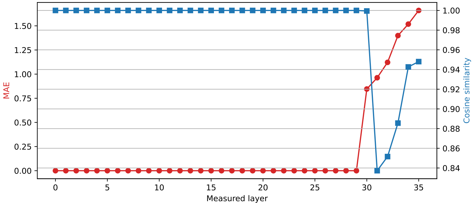
Qwen2.5-3B | Quantized layer 29 | float32 \rightarrow int4
