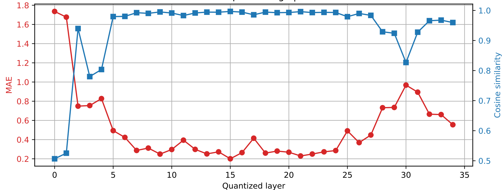
Qwen2.5-3B | Prompt 0 Final RMSNorm output damage | float32 \rightarrow int2
