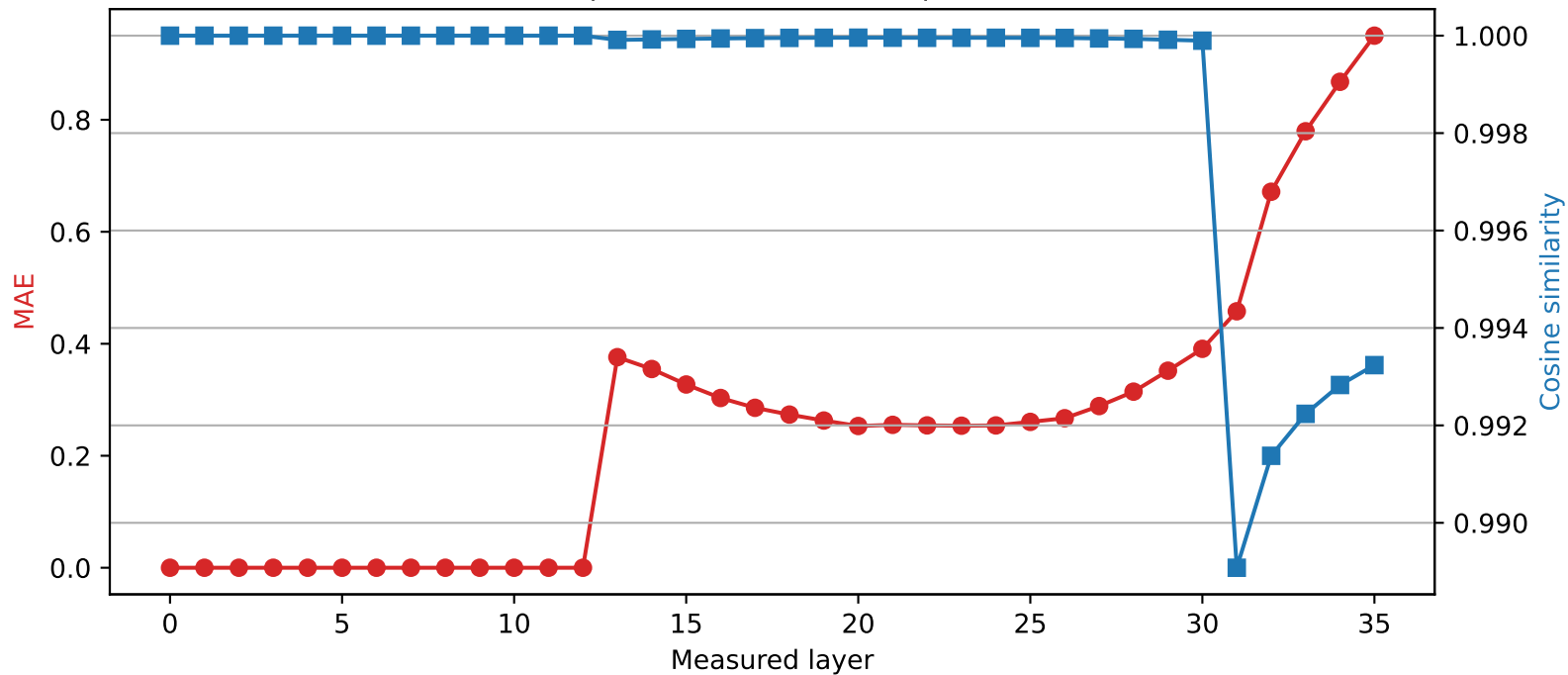
Qwen2.5-3B | Quantized layer 12 | float32 \rightarrow int2
