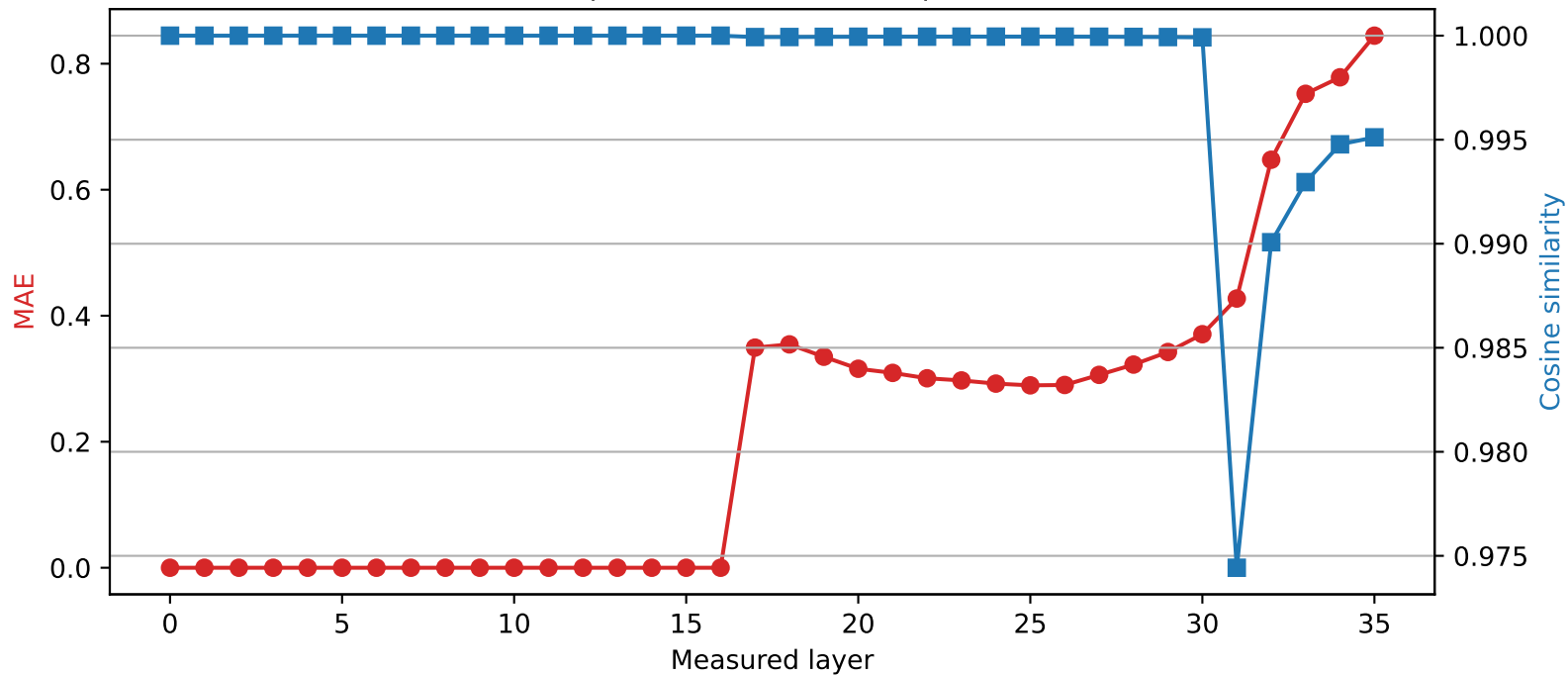
Qwen2.5-3B | Quantized layer 16 | float32 \rightarrow int2
