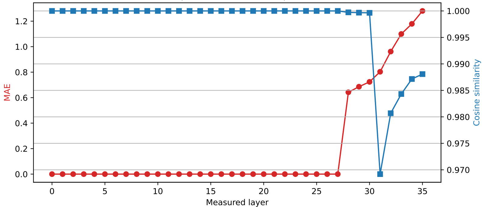
Qwen2.5-3B | Quantized layer 27 | float32 \rightarrow int2
