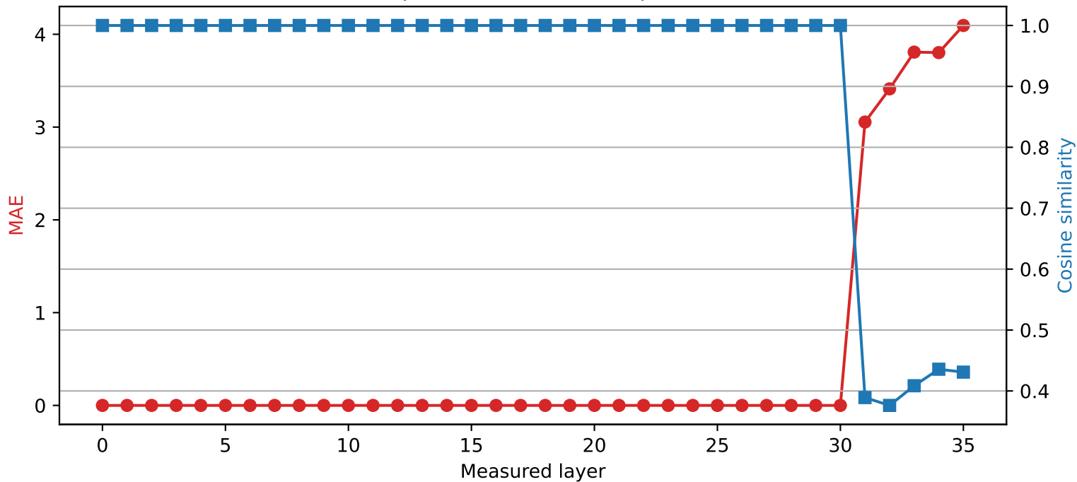
Qwen2.5-3B | Quantized layer 30 | float32 \rightarrow int2
