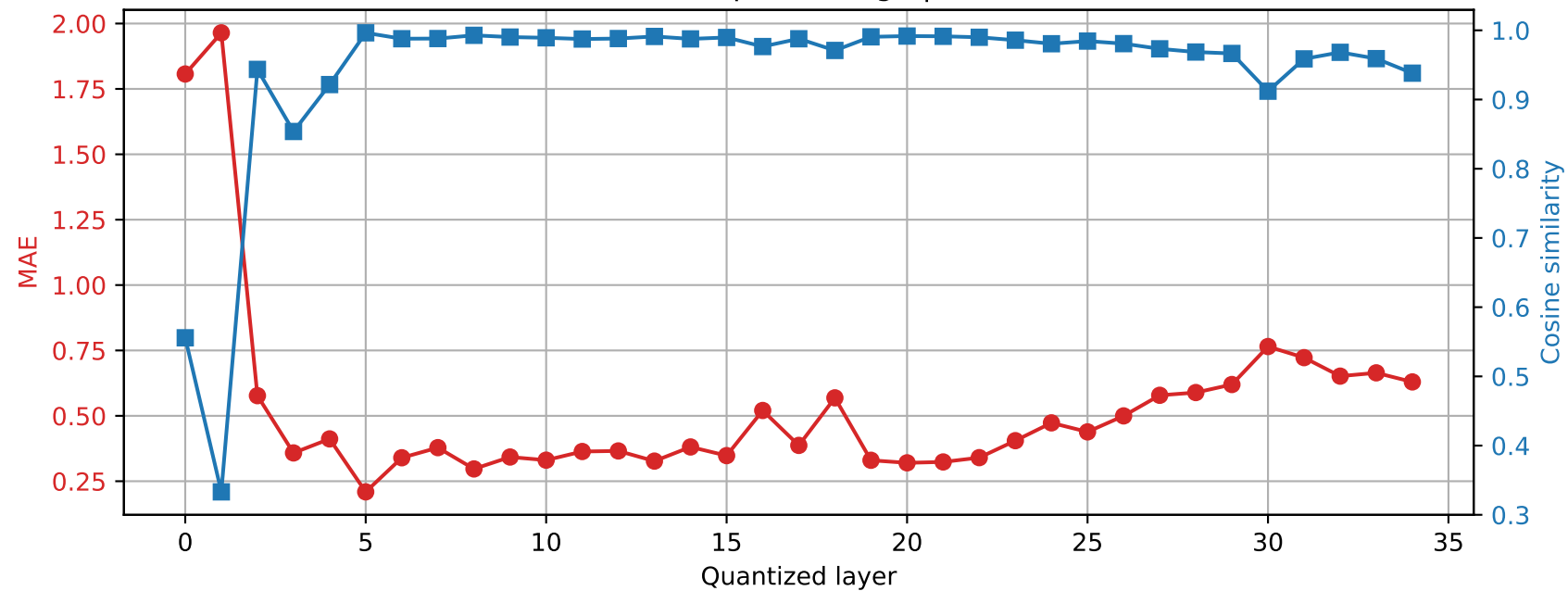
Qwen2.5-3B | Prompt 1 Final RMSNorm output damage | float32 → int2
