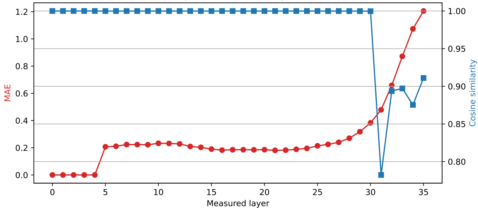
Qwen2.5-3B | Quantized layer 4 | float32 \rightarrow int2
