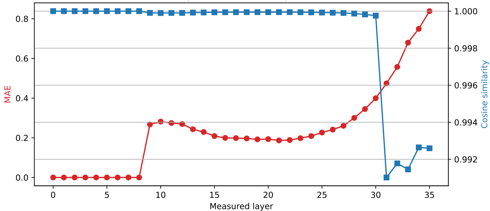
Qwen2.5-3B | Quantized layer 8 | float32 \rightarrow int2
