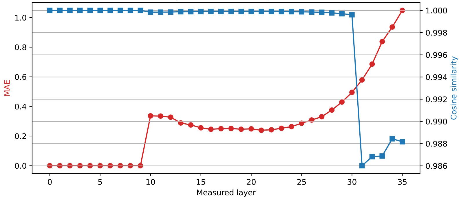
Qwen2.5-3B | Quantized layer 9 | float32 \rightarrow int2
