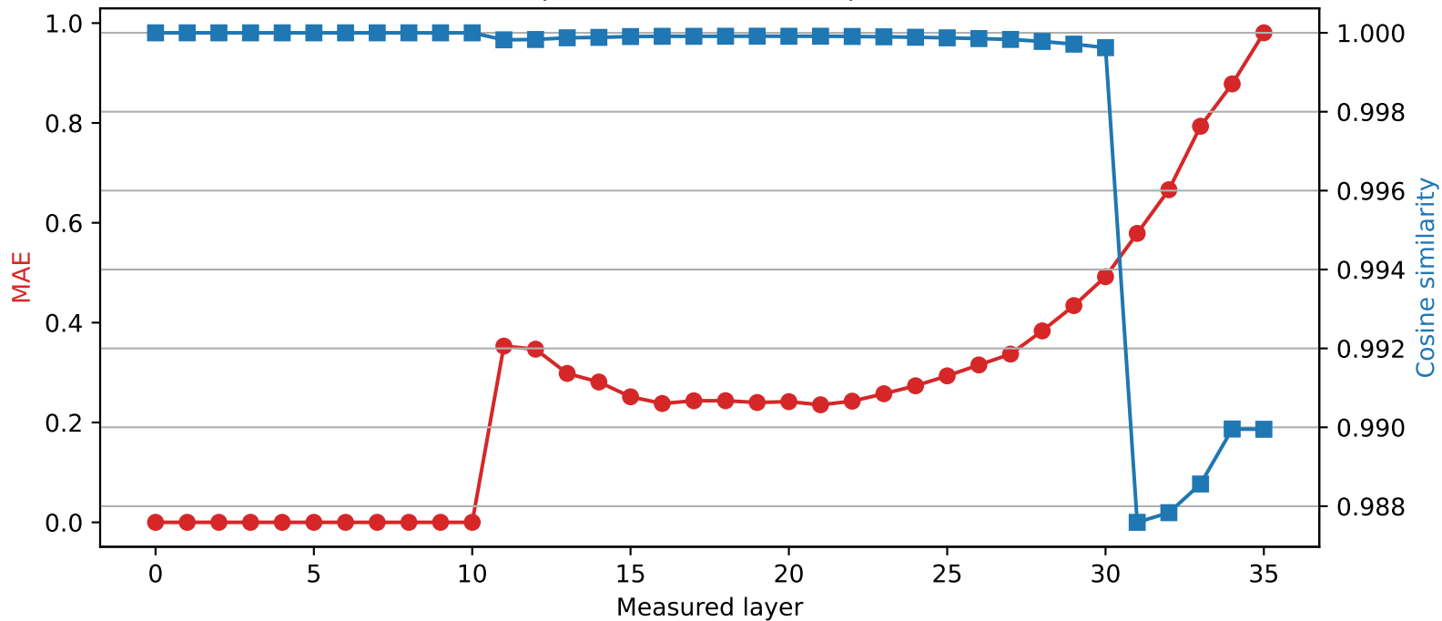
Qwen2.5-3B | Quantized layer 10 | float32 → int2
