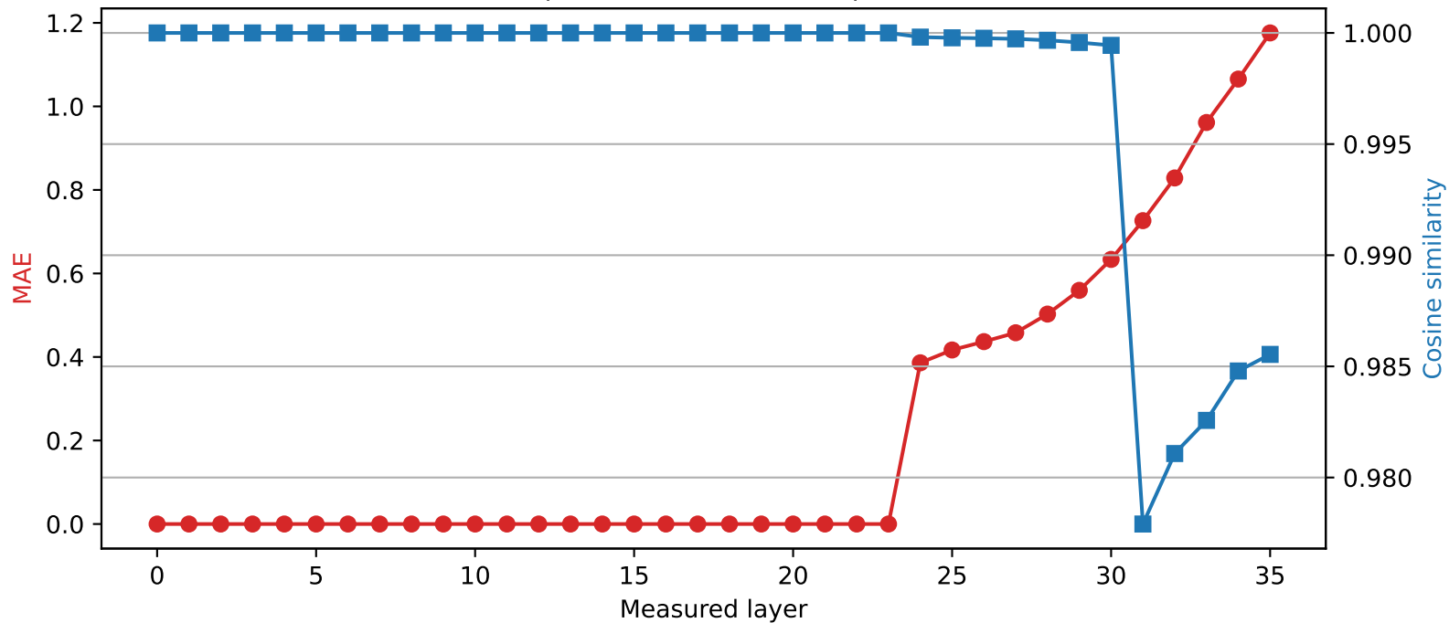
Qwen2.5-3B | Quantized layer 23 | float32 \rightarrow int2
