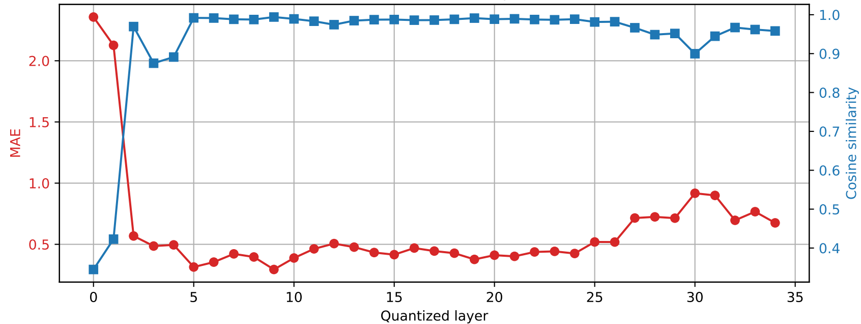
Qwen2.5-3B | Prompt 2 Final RMSNorm output damage | float32 \rightarrow int2
