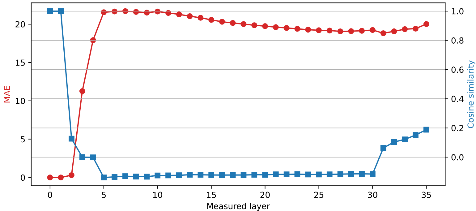
Qwen2.5-3B | Quantized layer 1 | float32 → int2
