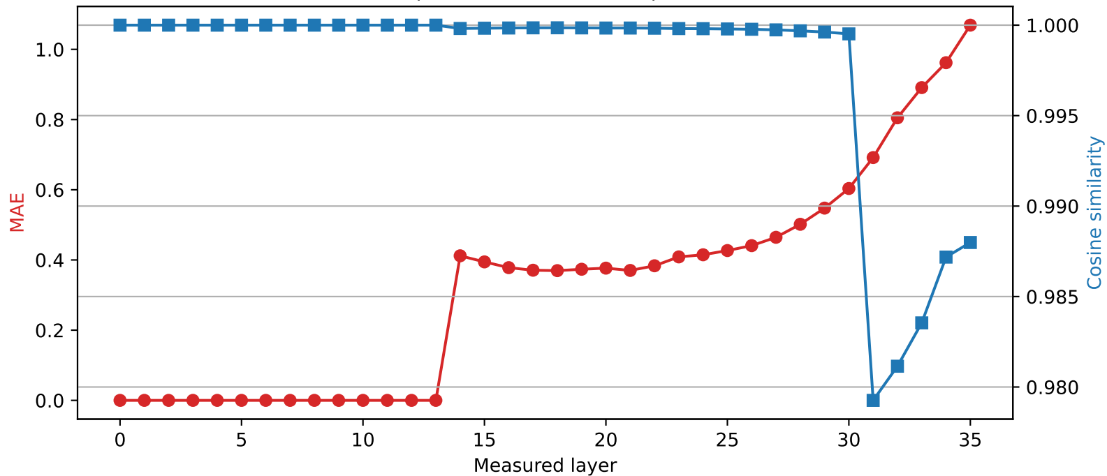
Qwen2.5-3B | Quantized layer 13 | float32 \rightarrow int2
