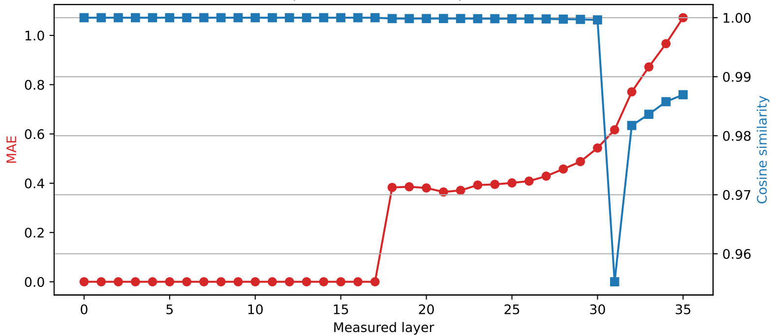
Qwen2.5-3B | Quantized layer 17 | float32 \rightarrow int2
