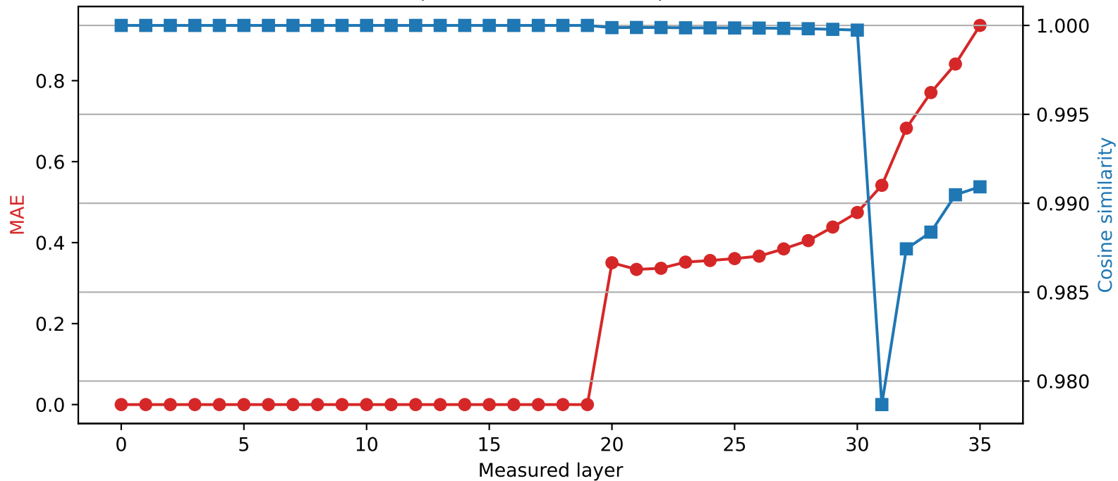
Qwen2.5-3B | Quantized layer 19 | float32 \rightarrow int2
