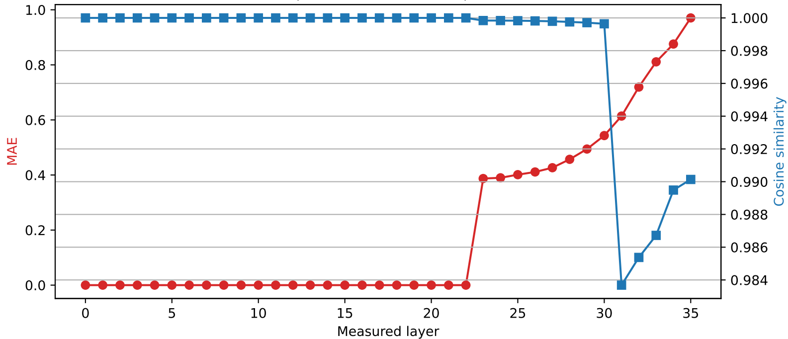
Qwen2.5-3B | Quantized layer 22 | float32 \rightarrow int2
